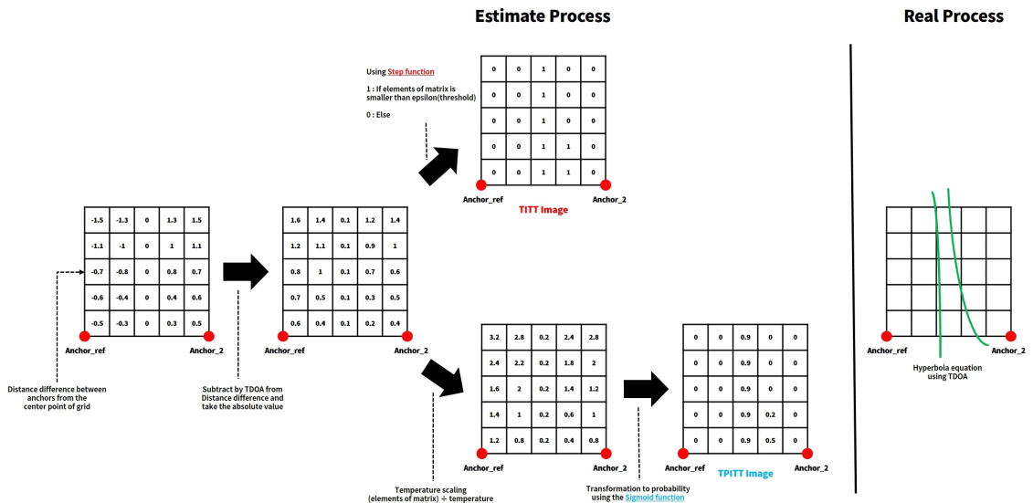
Fig. 2. Conversion of TDoA to image in TITT(upper, red) and TPITT(lower, blue).
